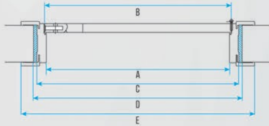
PICTURE 1: DOOR'S GENERAL CROSS SECTION
