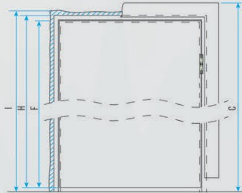
PICTURE 2: HEIGHT OF DOOR
