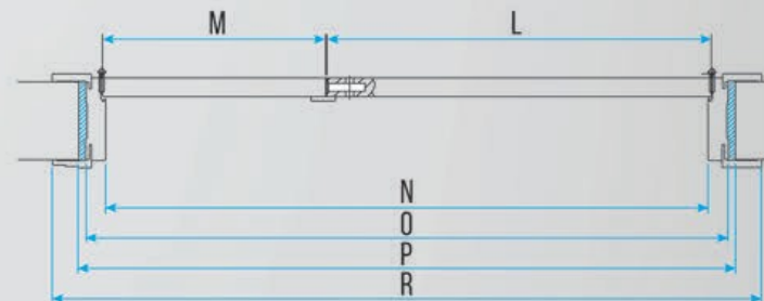
PICTURE 3: DOUBLE WING DOOR'S GENERAL CROSS SECTION
